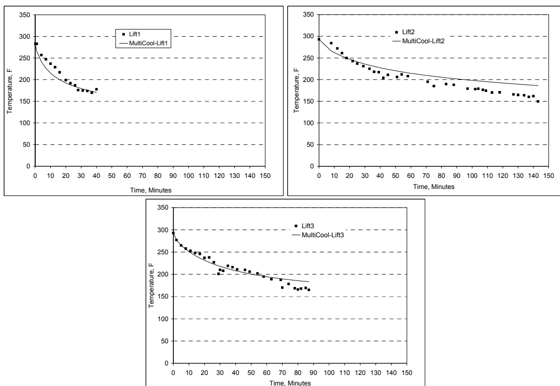
Figure 3.10 S12 (TLA) Measured and Predicted Cooling Curves (Lifts 1, 2 and 3)
