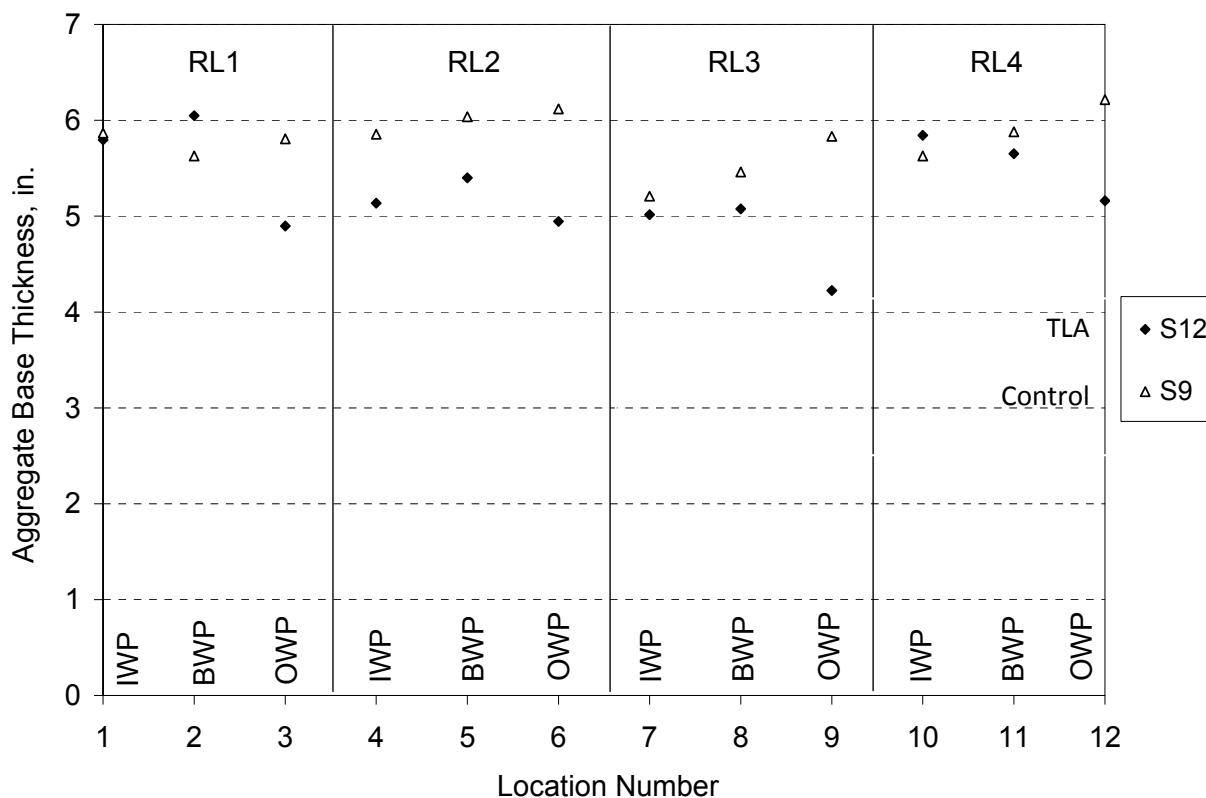
Figure 3.6 Surveyed Aggregate Base Thickness
