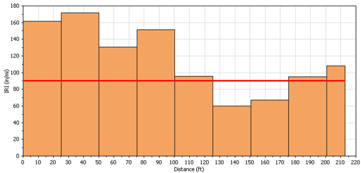
Figure 7.5 IRI – Right Wheelpath of S12
