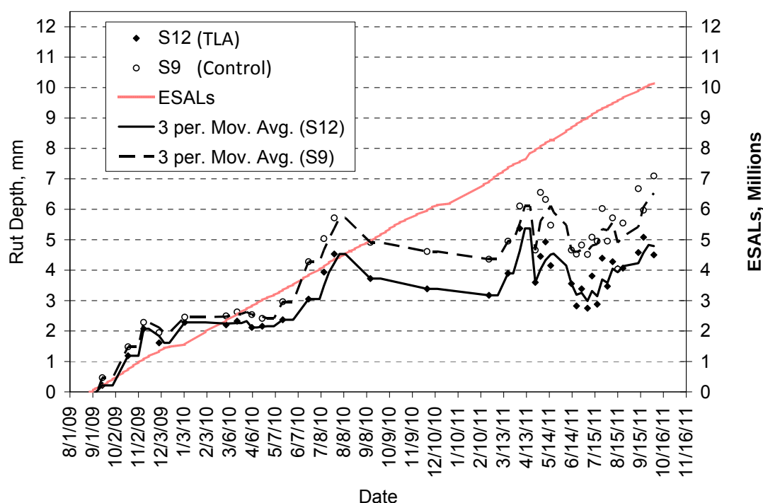
Figure 7.1 Measured Rut Depths - ARAN
