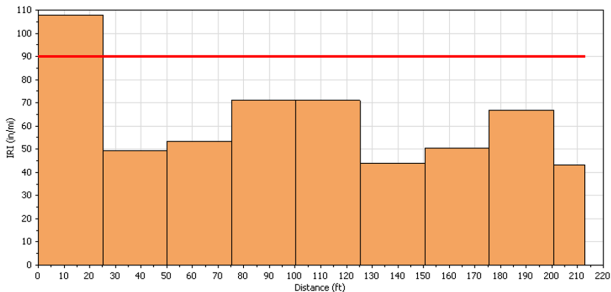
Figure 7.4 IRI – Left Wheelpath of S12
