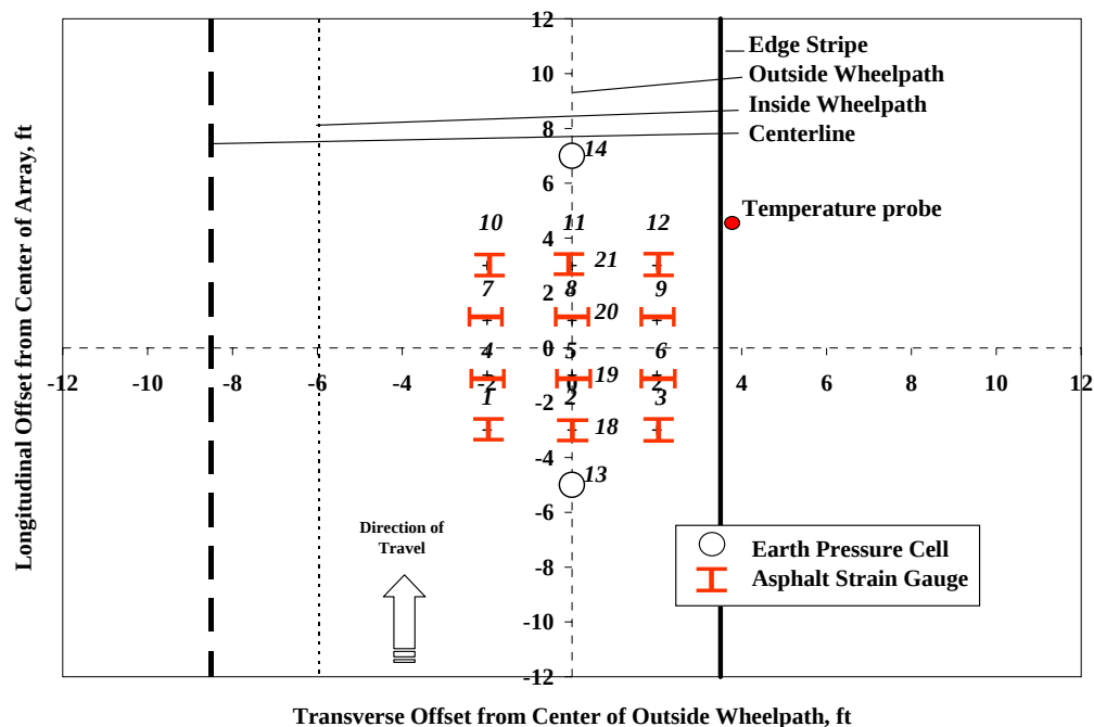
Figure 2.1 Gauge Array
