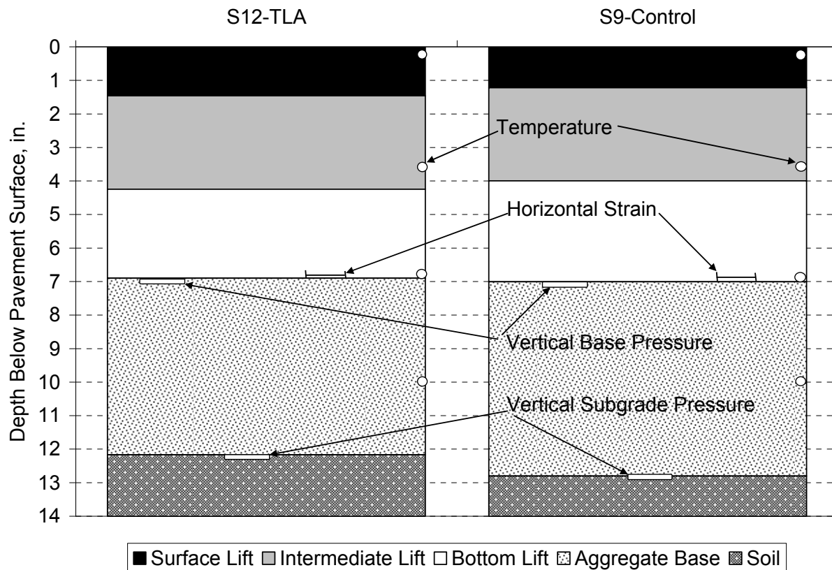
Figure 3.12 Average Lift Thicknesses and Depth of Instrumentation
