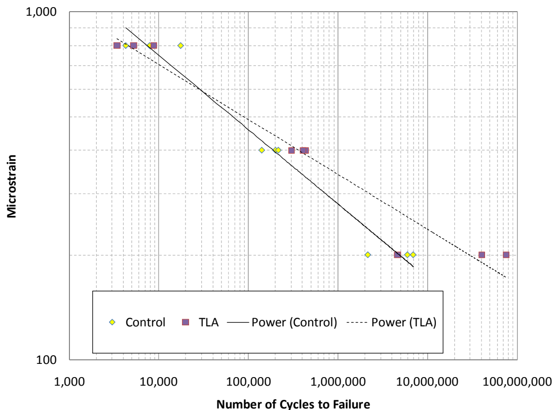
Figure 4.9 Comparison of Fatigue Resistance for Mixtures
